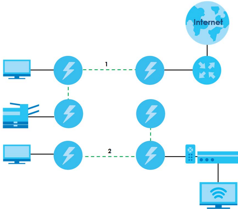
Figure 25 Add New Adapters to Make a Second Network
