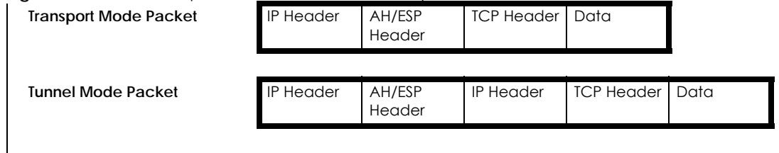
Figure 327 VPN: Transport and Tunnel Mode Encapsulation
