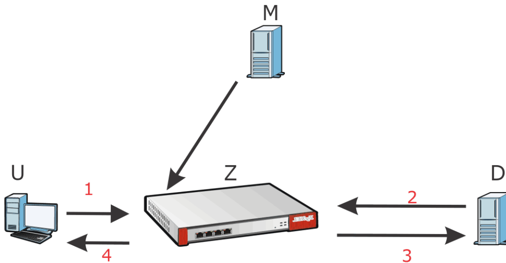
Figure 429 SSL Inspection Certificate Update Overview
