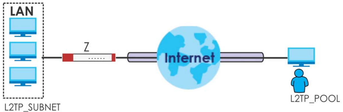
Figure 335 Policy Route for L2TP VPN
