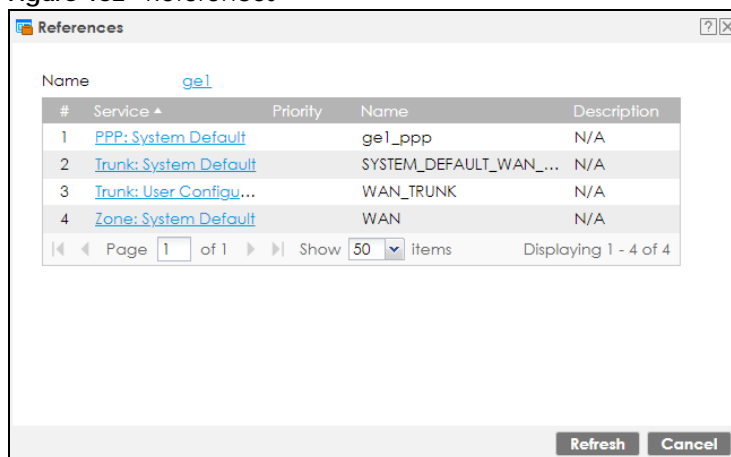
Figure 182 References
