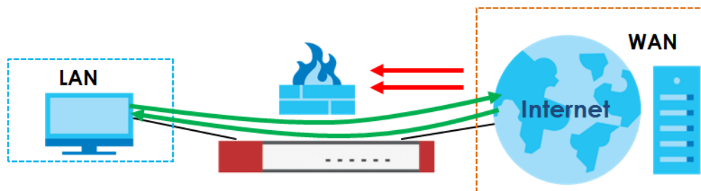
Figure 399 Default Directional Security Policy Example
