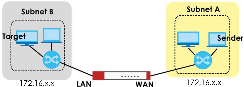
Figure 179 Proxy ARP
