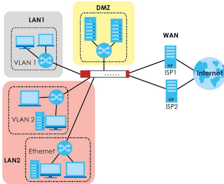
Figure 435 Example: Zones
