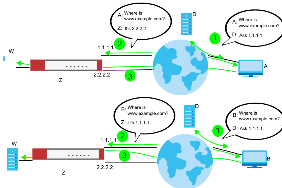
Figure 307 DNS Load Balancing Example
