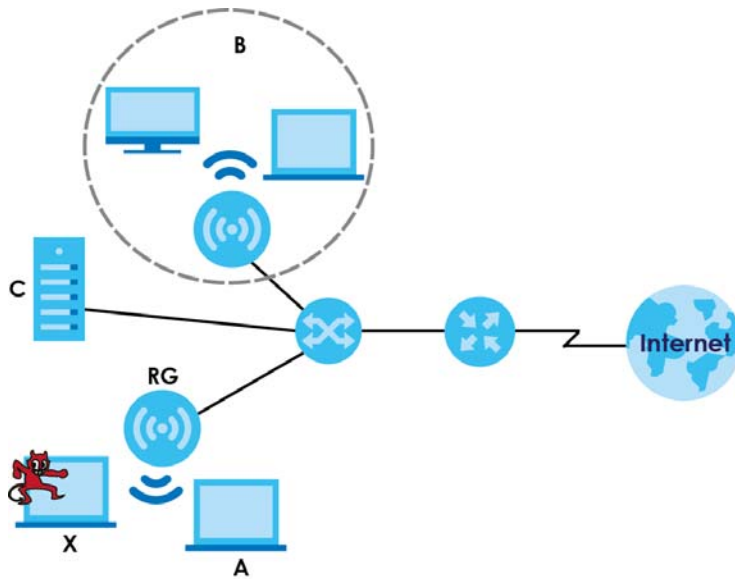
Figure 468 Rogue AP Example
