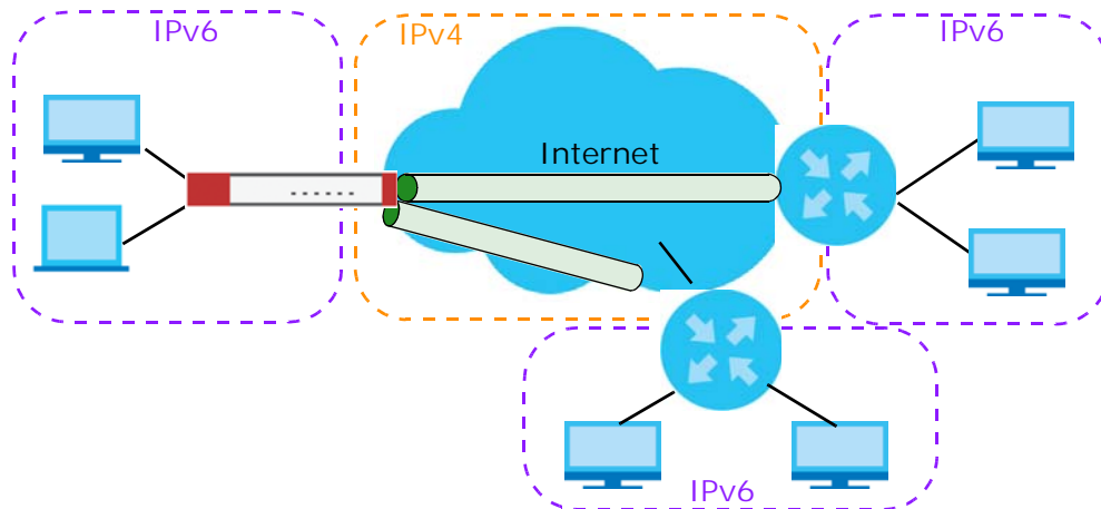
Figure 193 6to4 Tunnel
