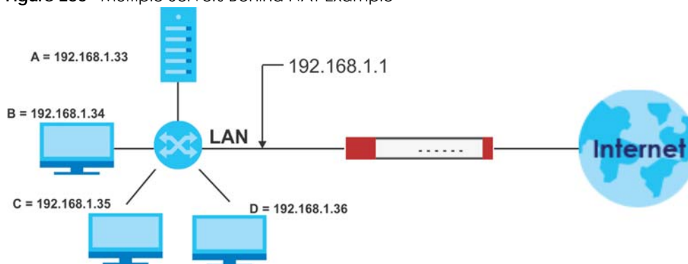
Figure 236 Multiple Servers Behind NAT Example
