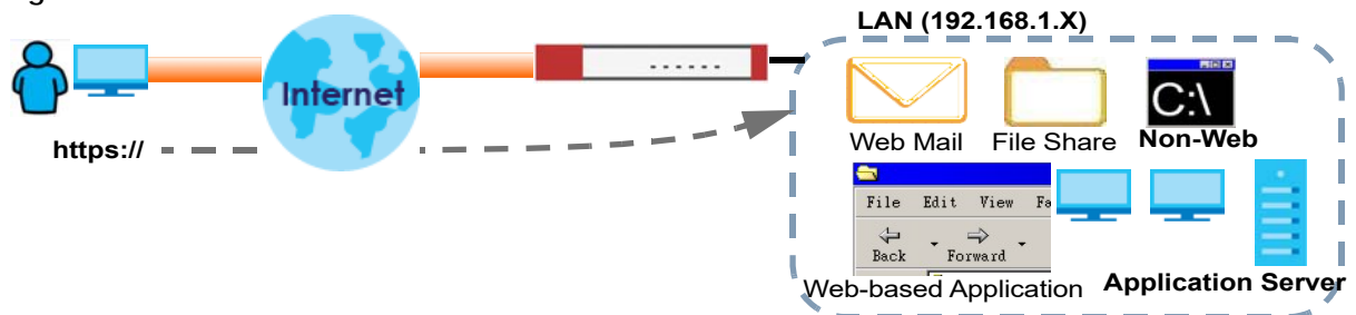
Figure 312 SSL VPN
