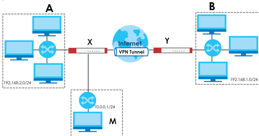
Figure 328 VPN Example: NAT for Inbound and Outbound Traffic
