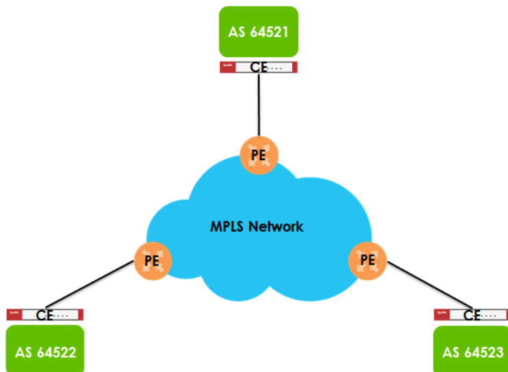
Figure 232 Scenario 1: CE Router - to - MPLS
