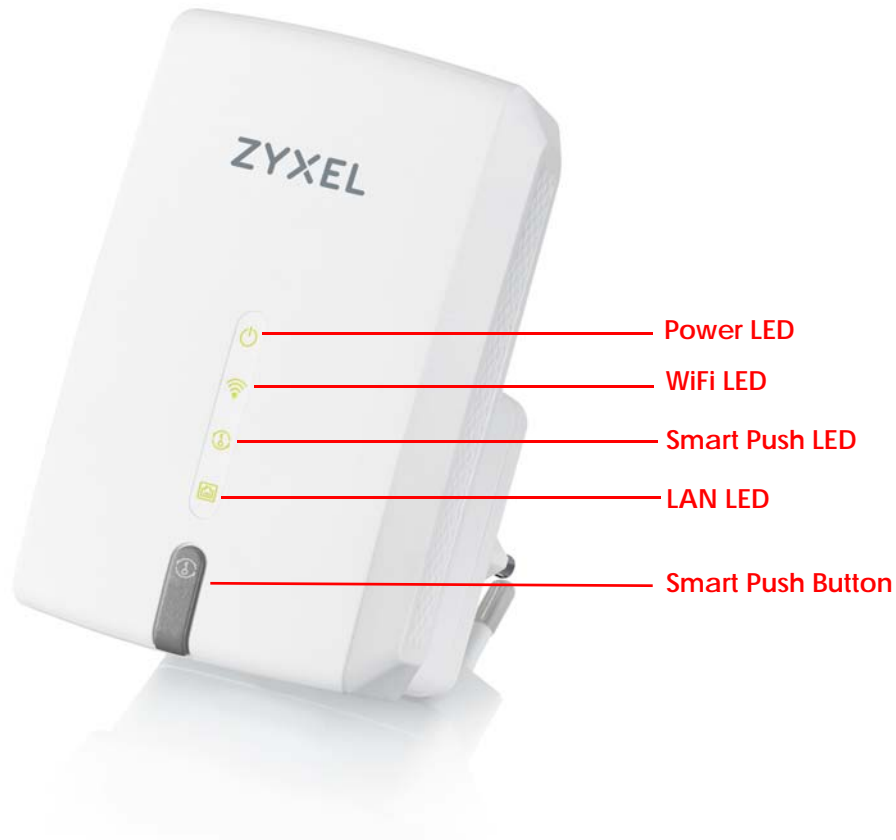
Figure 3 Front Panel
