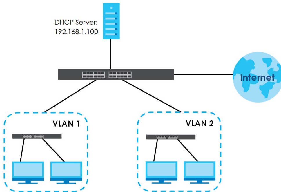
Figure 182 Global DHCP Relay Network Example
