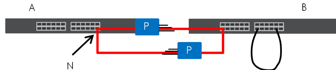
Figure 261 Loop Guard – Probe Packet
