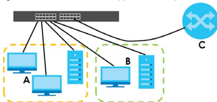
Figure 99 Protocol Based VLAN Application Example
