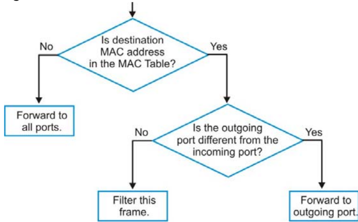
Figure 288 MAC Table Flowchart
