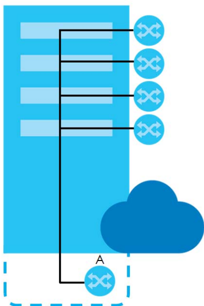
Figure 283 Clustering Application Example
