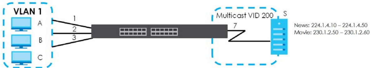
Figure 165 MVR Configuration Example
