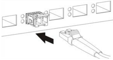
Figure 19 Connecting the Fiber Optic Cables
