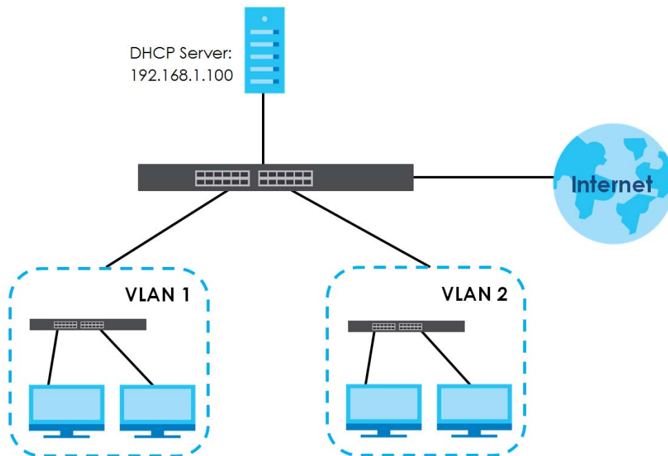
Figure 243 Global DHCP Relay Network Example
