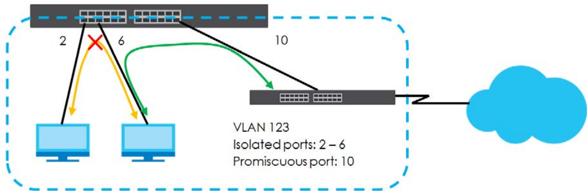
Figure 208 VLAN Isolation Example
