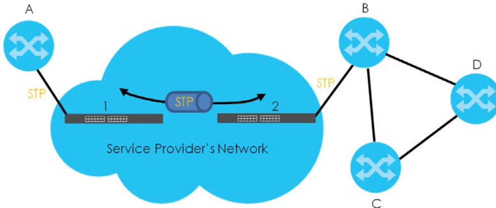
Figure 196 L2PT Network Example
