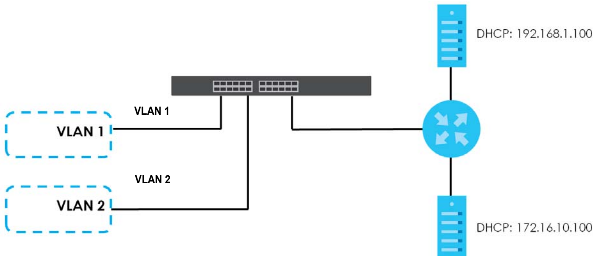
Figure 247 DHCP Relay for Two VLANs
