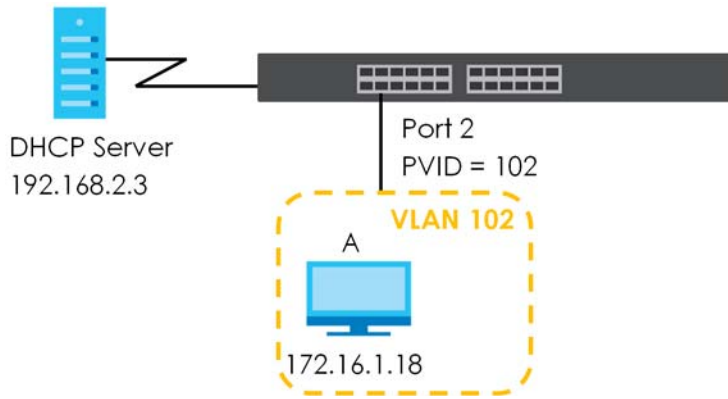
Figure 54 Tutorial: DHCP Relay Scenario
