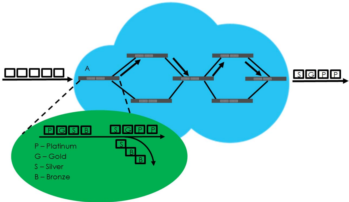
Figure 235 DiffServ Network
