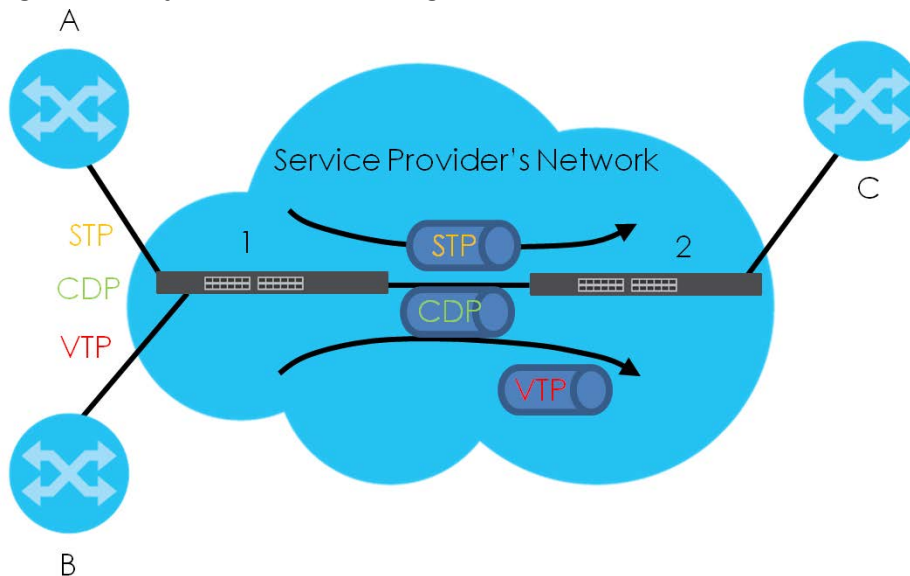
Figure 195 Layer 2 Protocol Tunneling Network Scenario
