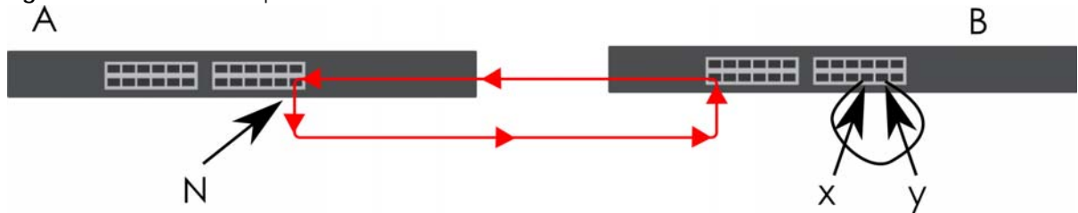
Figure 191 Switch in Loop State
