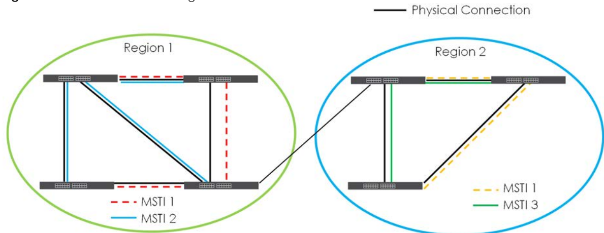
Figure 123 MSTIs in Different Regions
